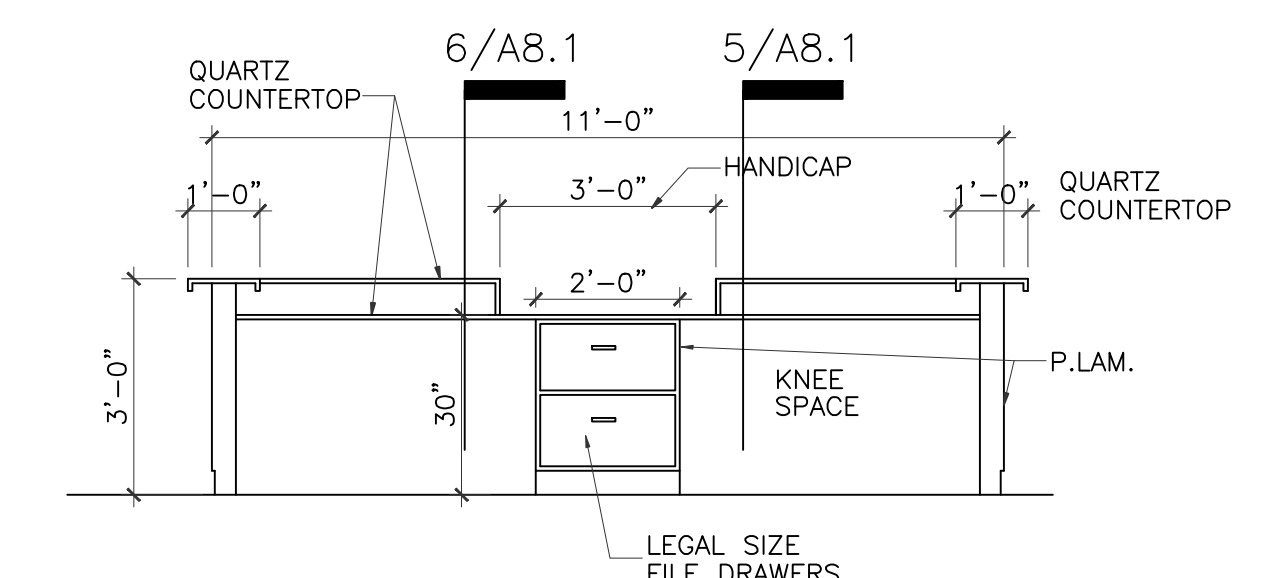
11 MILLWORK ELEVATION-RECEPTION 3/8" = 1'-0"
