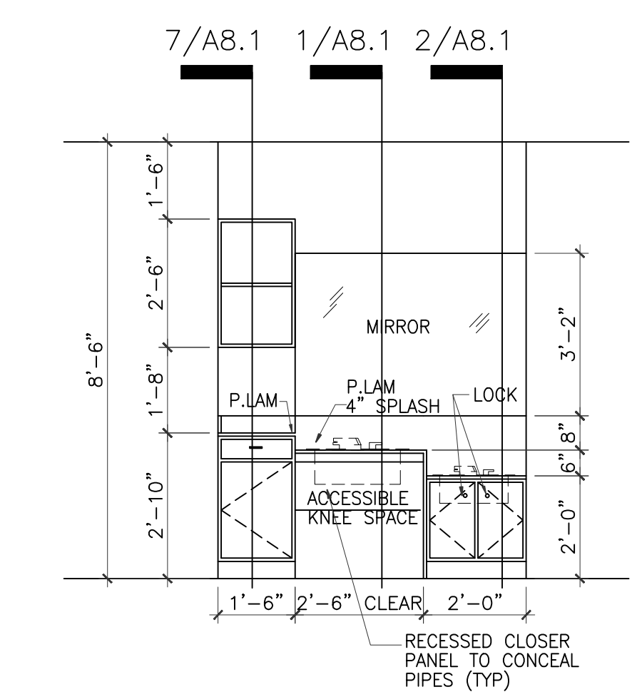
5 MILLWORK ELEVATION 3/8" = 1'-0" CLASSROOM #250
