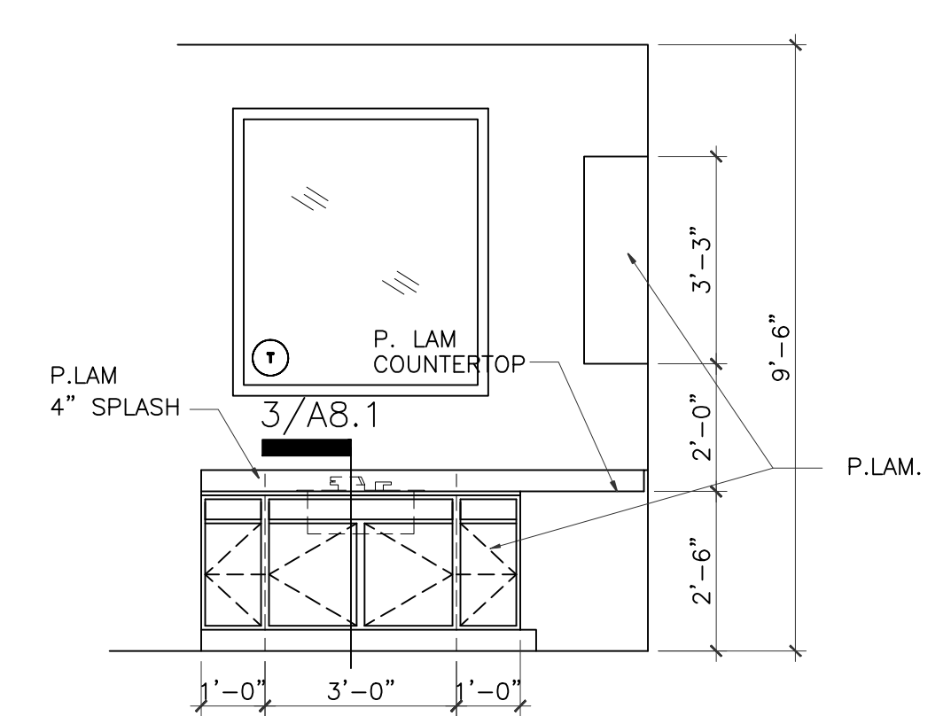
14 MILLWORK ELEVATION-ACTIVITY 3/8" = 1'-0"
