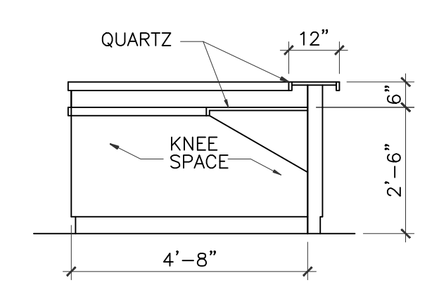
9 MILLWORK ELEVATION-RECEPTION 3/8" = 1'-0"
