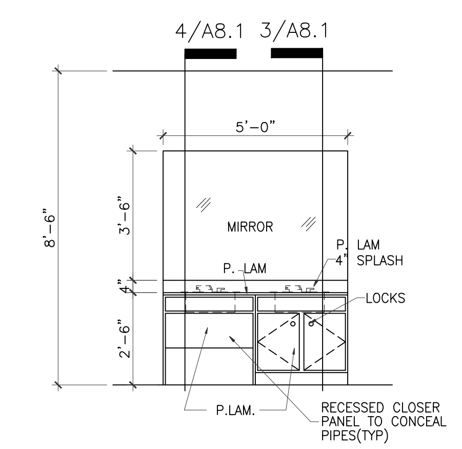
16 MILLWORK ELEVATION 3/8" = 1'-0" CLASSROOM #400 CLASSROOM #450 CLASSROOM #500 CLASSROOM #550 ACTIVITY ROOM
