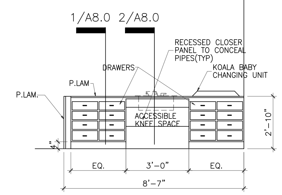
4 MILLWORK ELEVATION 3/8" = 1'-0" CLASSROOM #100 CLASSROOM #150 (OPP. HD.) CLASSROOM #200
